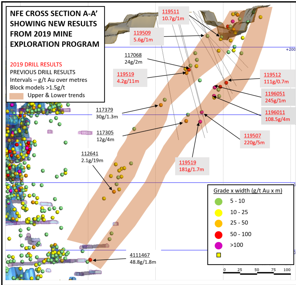
Figure 3. Cross section of high-grade zones at NFE
