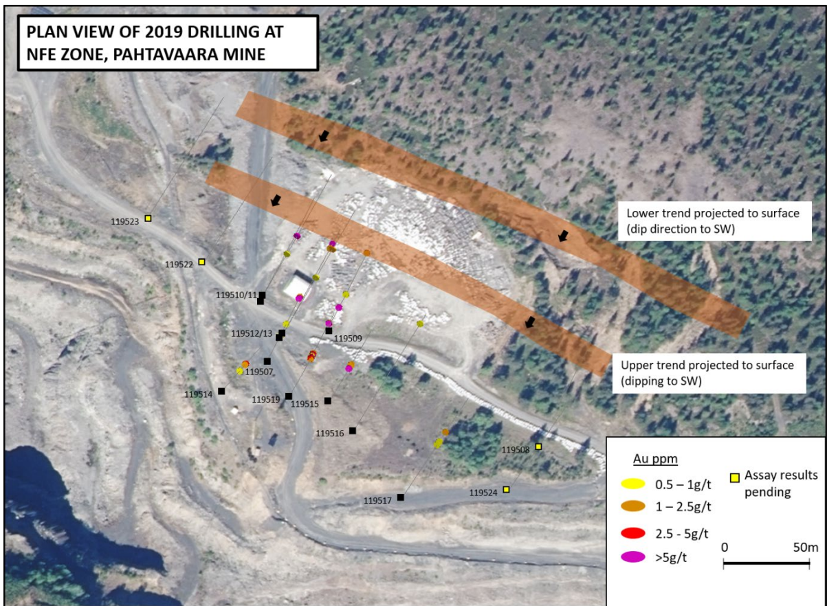
Figure 2. Plan view of recent NFE drilling and projection of Upper and Lower mineralised trends.
